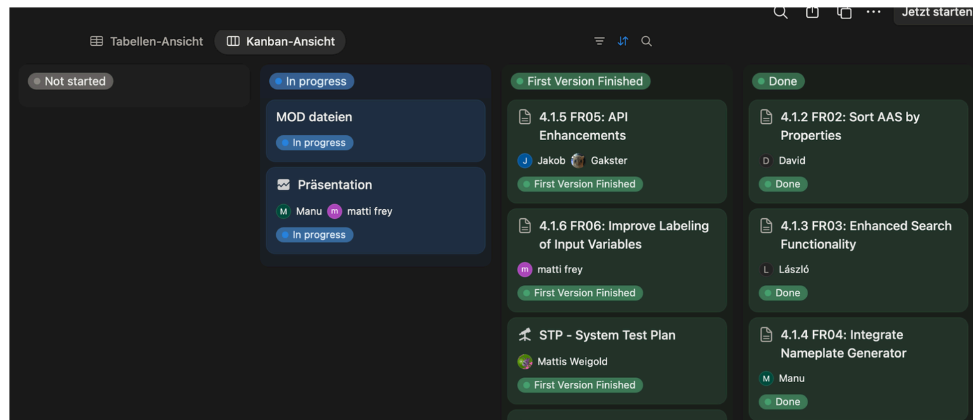
Fig. 22: Kanban board
